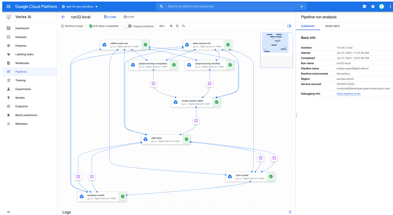
Vertex_AI_Pipeline
